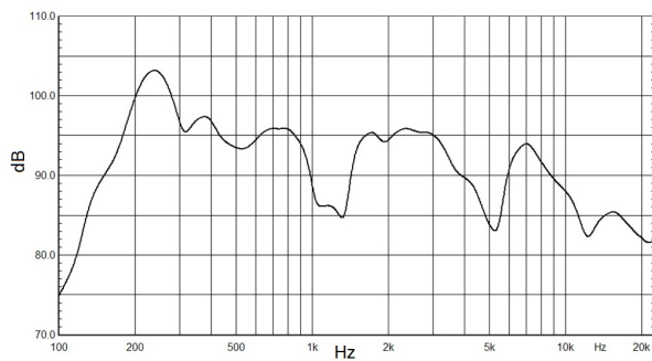
Frequency Response
