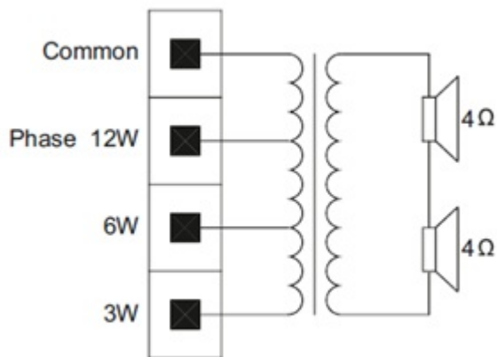
Circuit Diagram
